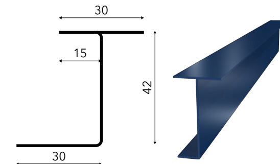
AKUSTILINE URBAN TL42
